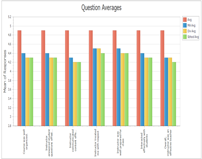
Calc 3, Spring 2016
