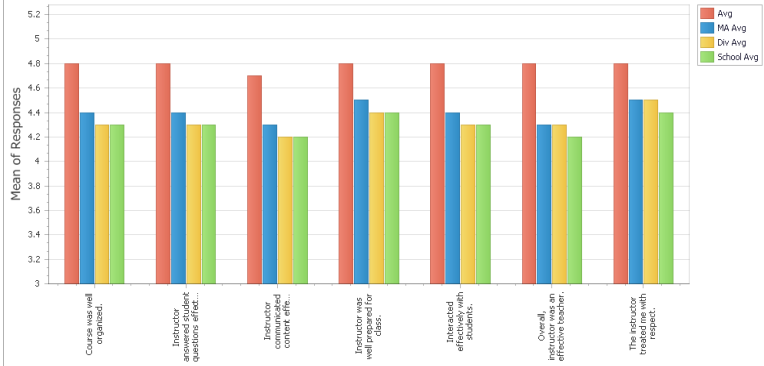
Question Averages
