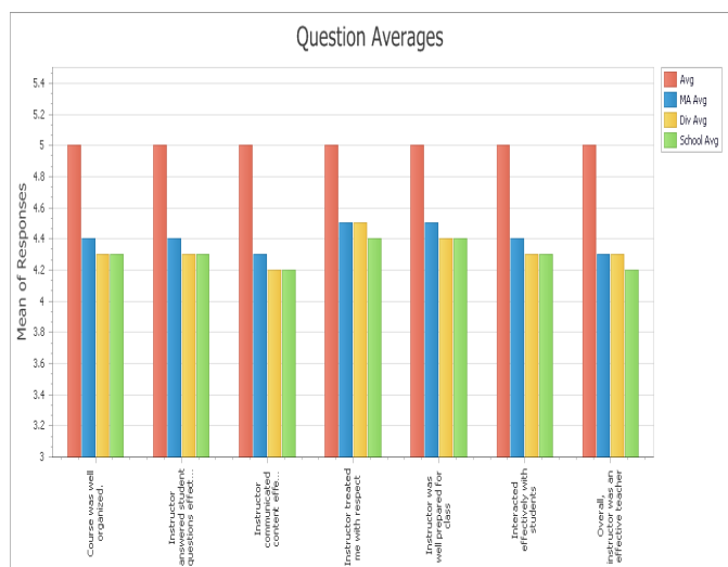
Calc 3, Fall 2015
