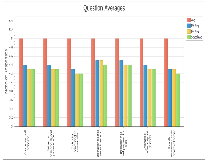
Calc 3, Spring 2016
