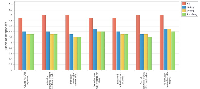
Question Averages
